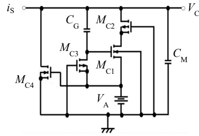
Fig. 4. Circuit diagram of the cell body model.
