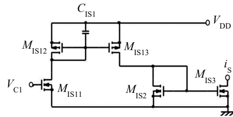
Fig. 5. Circuit diagram of the inhibitory synaptic model.
