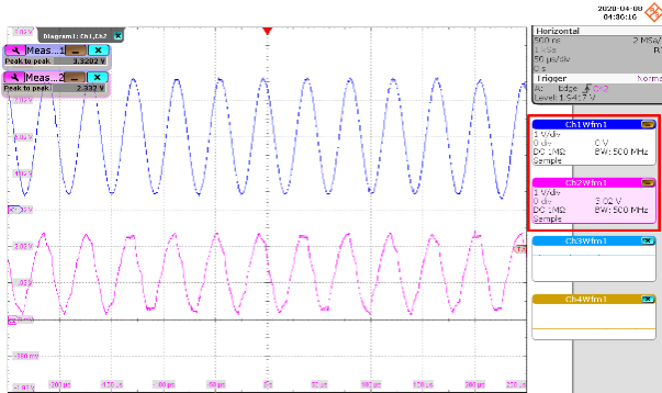
Fig. 8. Bandwidth measurement
