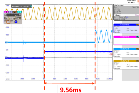
Fig. 3. The latency of input to output
