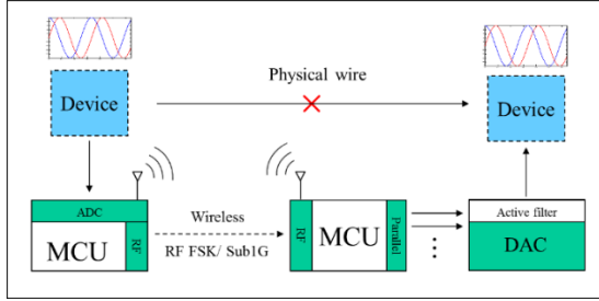
Fig. 1. The figure of system architecture
