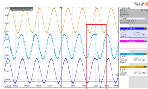
Fig. 4. The situation of hardware switching As shown in Fig. 4, the experiment is performed to measure this non-updating duration. In every 43.75us of transmission frame, there is about 3.2 ms of non-working interval.
