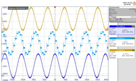
Fig. 2. The comparison of whole system output and input result In the oscilloscope waveform of Fig. 2, Ch4 (brown curve) is the waveform produced by the function generator; Ch3 (light blue curve) is the output after DAC; and Ch1 (indigo curve) is the result of the filter which is also the signal after the reconstruction. The Fig. 2 shows that the 16 kHz sinusoidal wave input signal can be reconstructed by 10 digital data.
