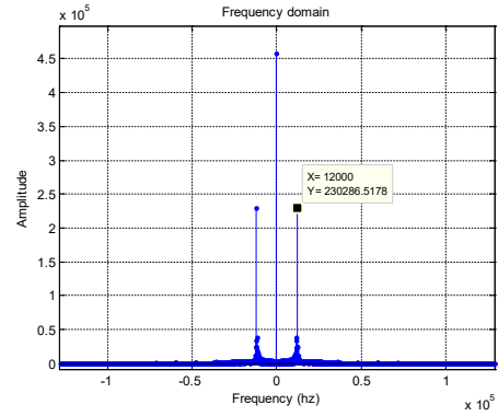
Fig. 7. The frequency domain figure of output result
